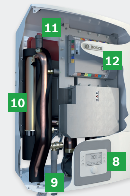
AWE indoor unit
