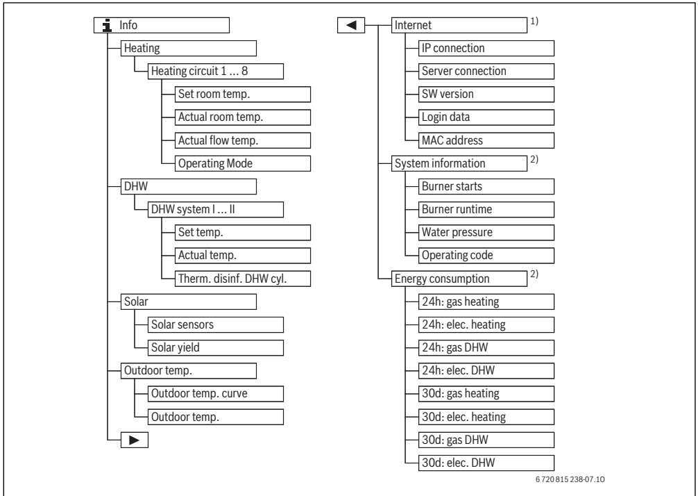
Fig. 5 Menu structure of the info menu
